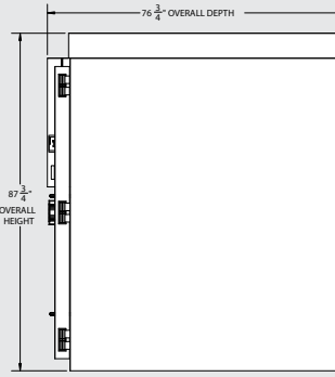
BF202DP-1P / BF202AP-1P
